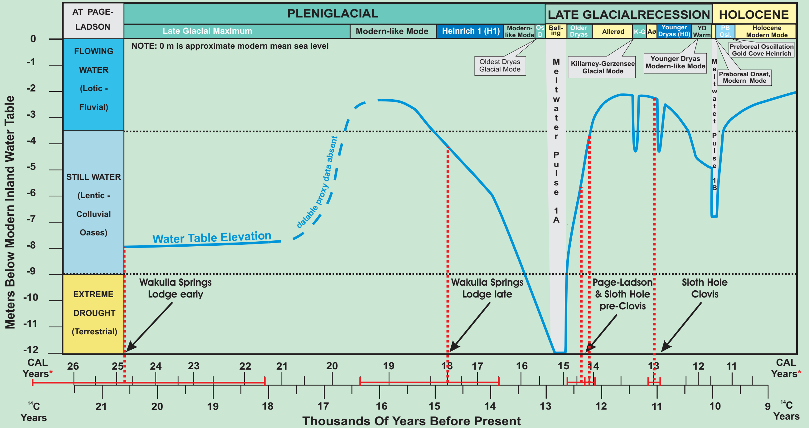
Pleistocene Water Table Fluctuations In North Florida Based On Data From The Page-Ladson Site Also Showing Global & Regional Climate Events & Dated Paleoindian Components
